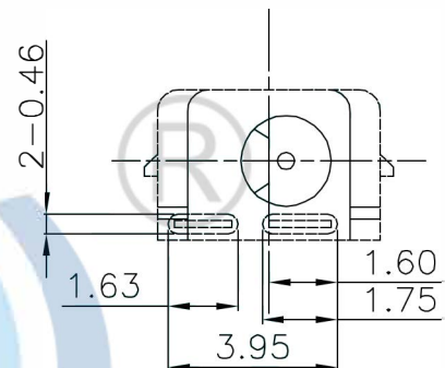
P.C.B LAYOUT (front view)
